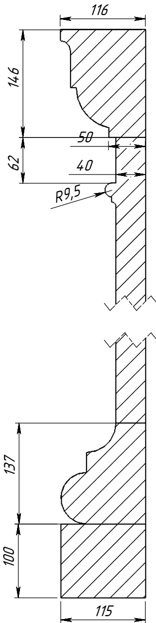
SECTION E-E SCALE 1 : 5
