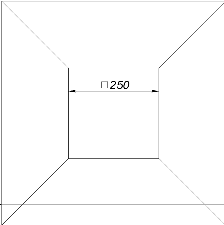
DETAIL E SCALE 2 : 5
