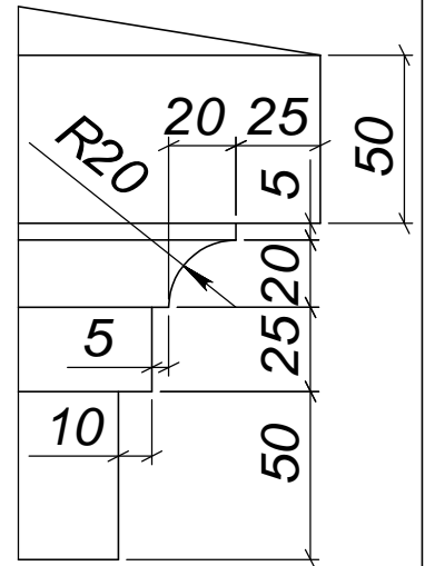
DETAIL E SCALE 2 : 5
