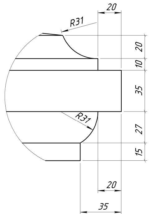
DETAIL E SCALE 1:2
