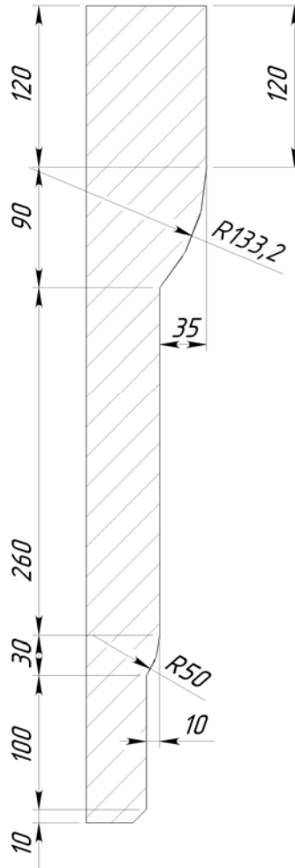
SECTION F-F
